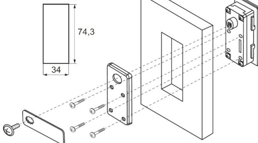
Drilling template for wooden panel
